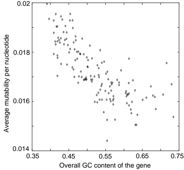
Figure 4.1: Average nucleotide mutability versus the G/C content of the sequence. Each data point represents one non-immunoglobulin sequence.
