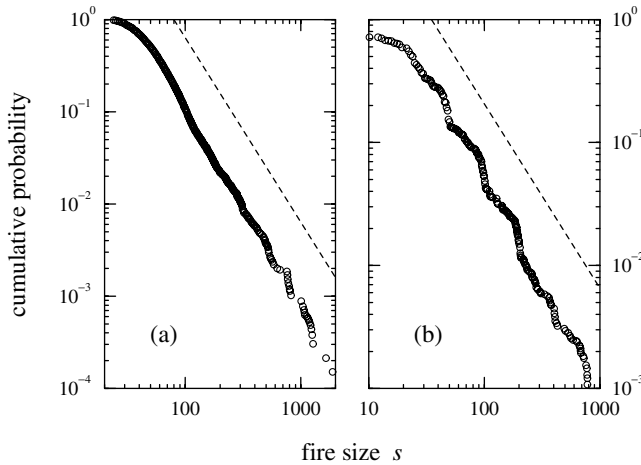
FIG. 1. Cumulative distribution of fire sizes for simulations of the forest fire model in one and two dimensions, plotted on logarithmic scales. (a) One dimension with size 10000 and an exponential spark distribution. (b) Two dimensions with size 128 \times 128 and a Gaussian spark distribution. The results have been averaged over a number of different values of the parameters of the spark distributions to improve the statistics. The dotted lines show the expected slopes of -2 and -\frac{3}{2} .
