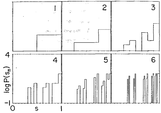
Fig. 13. P_\infty for the logistic equation (19) with r=3.7 , taken from [27]. The interval is partitioned into two equal parts, which are assigned the symbols 0 and 1. Symbol sequences S_m = .s_1 s_2 \dots s_m are generated by iterating the map, and binned to approximate P(S_m) . Successive approximations to P_\infty are shown in the figure. The metric entropy is the information dimension of P_\infty , and the topological entropy is the fractal dimension (using \log_2 ).
