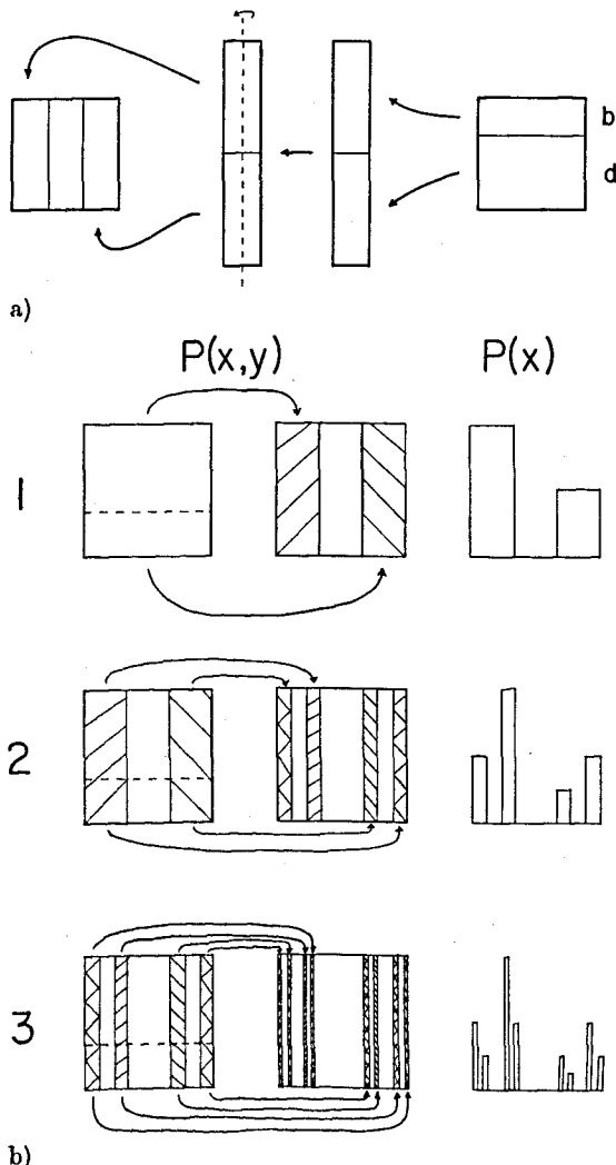
Fig. 4. (a) A geometric illustration of Yorke's Map. (b) Successive iterations of the map act on an initially uniform probability density as shown. The attractor is the Cartesian product of the classic Cantor set and the interval. The information dimension is given by (16).
