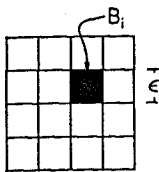
Fig. 1. A schematic drawing of a uniform two dimensional partition. \epsilon is the minimum scale of resolution, and B_i is an element of the partition, corresponding to the outcome of a measurement.
