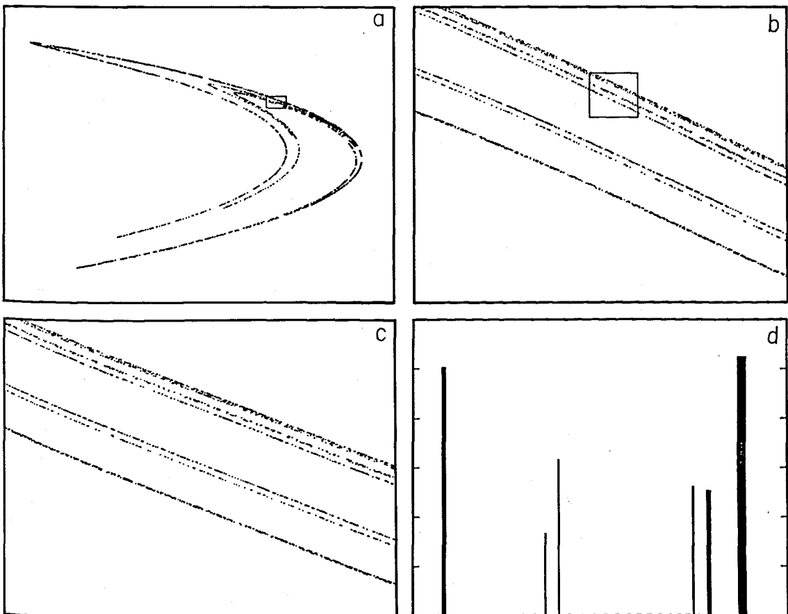
Fig. 5. The Henon attractor, see Equation (17). Figures 5(b) and 5(c) show successive blowups of the regions inside the box of the previous figure. Resolving the fractal structure of Fig. 5(c) into six "leaves", the relative probabilities of these leaves are plotted in Figure 5(d). The width of each bar is roughly the width of the corresponding leaf. This unequal distribution of probabilities persists on all scales, making the Henon attractor a "measure fractal".
