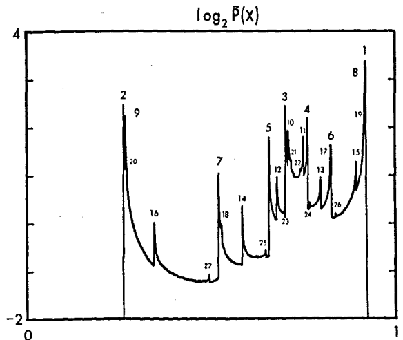
Fig. 8. The asymptotic probability distribution \{\bar{P}_i\} for the logistic equation x_{i+1} = 3.7 x_i (1 - x_i) , obtained by iterating 10^8 times and binning the result into 1000 bins. The corresponding density \bar{P}(x) contains an infinite number of integrable discontinuities, labeled in the figure according to the iterate from the critical point. Their amplitude decreases roughly exponentially. The information dimension D_1 = 1 .
