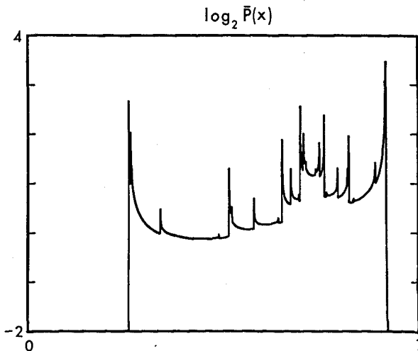
Fig. 10. The approximation to P(x) given in (20).
