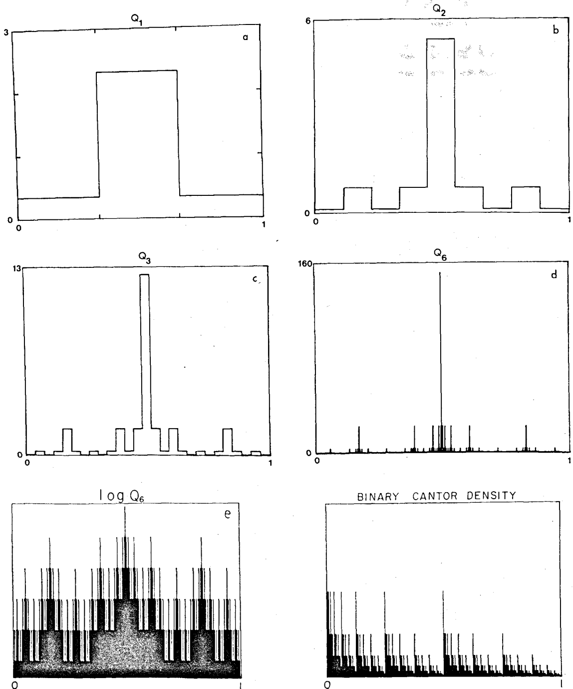
Fig. 2. "Cantor's density" has an information dimension D_1 = \log 2 / \log 3 , but the fractal dimension of its support is 1 (see Eq. (12)). (a) Q_1(x) = 3p_0 \cong 0.3406 on (0, 1/3) and (2/3, 1) , and Q_1(x) = 3p_m \cong 2.3187 on (1/3, 2/3) . Using a uniform three piece partition, the information I(1/3) is one bit. (b) To form Q_2 , the probabilities are redistributed among 9 pieces (see Eq. (7), i = 2 ). Using the 3^2 element partition, I = 2 bits. (c) i = 3 , I = 3 bits. (d) i = 6 . Because of the finite linewidth of the plotter, this is indistinguishable from the limiting case except for the vertical scale (in the limit the spikes become infinite).
