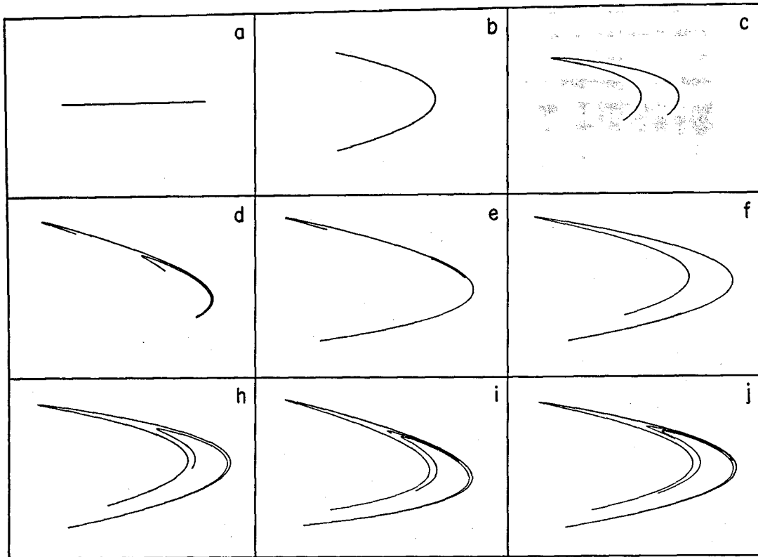
Fig. 6. Successive iterates by the Henon map of the line segment shown in Figure 6a. The spacing between the folds that form after several iterations is not constant; when evaluated at a finite level of resolution unequal numbers of them appear to merge, yielding the probability structure seen in Figure 5(d).
