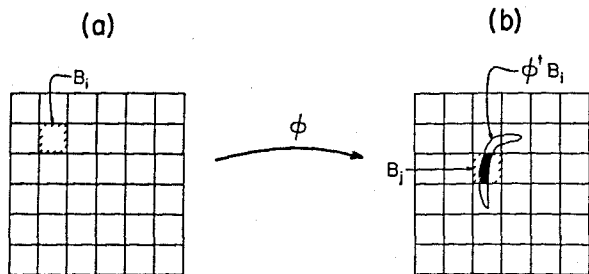
Fig. 15. (a) Assume that an initial measurement finds that the state is contained in partition element B_i . (b) Given outcome B_i at time 0, a time t later the state must be somewhere inside \phi^t B_i ; the probability that a measurement at time t will have outcome B_j is \bar{\mu}(B_j \cap \phi^t B_i) , where \bar{\mu} is the invariant measure (which gives the proper a priori weight to each outcome).
