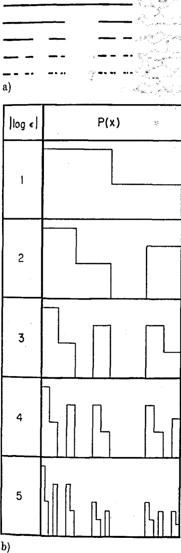
Fig. 7. (a) Successive approximations to an asymmetric Cantor set, formed by deleting the third fourth of each continuous piece. (b) Assuming the initial probability density of points on the interval is uniform, the coarse grained probability distribution is evaluated at successively finer scales of resolution \epsilon = 2^{-i} , i = 1, 2, \dots, 5 .
