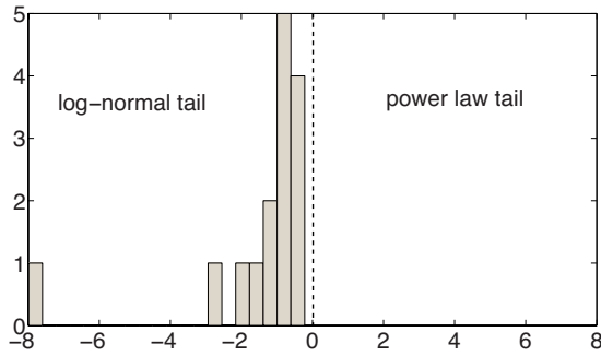
FIG. 3. (Color online) A histogram of the base 10 log likelihood ratios \mathcal{R} computed using Eq. (3) for each of the years from 1991 to 2005. A negative log likelihood ratio implies that it is more likely that the empirical distribution is log-normal than a power law. The log likelihood ratio is negative in every year, in several cases strongly so.
