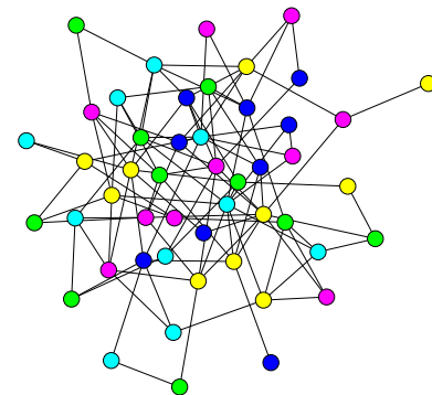
disassortative communities
