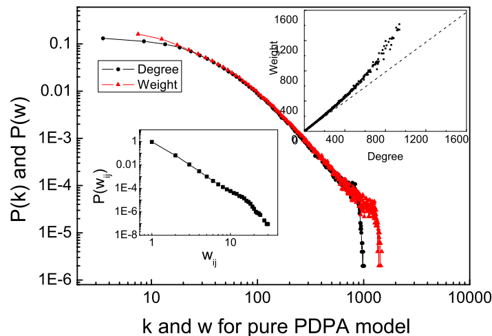
Figure 6. The model with pure \delta mechanism demonstrates all the typical power-law distributions with a high clustering coefficient as shown in the top curve in figure 5. The top-right inset is the correlation between vertex weight and vertex degree, with \eta = 1.19 . The bottom-left inset is the distribution of edge weight.
