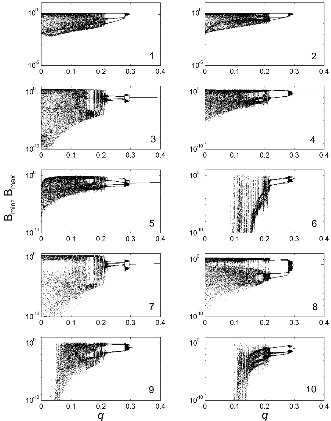
Figure 6. Local minima and maxima for each species in the ten-species food web shown in figure 4 for a range of values of q . Each panel is labeled with the species number, species 1 and 2 are the producer species. Note the use of a log axis to show in more detail the behavior of the minima. The non-zero parameter values are x_{3-10} = .2 ; y_{ij} = 2.5 for i = 3-6 , y_{ij} = 5 for i = 7-10 ; a_{31} = a_{32} = a_{41} = a_{42} = .5 , a_{51} = 1 , a_{63} = a_{64} = .5 , a_{73} = 1 , a_{84} = a_{85} = .4 , a_{86} = .2 , a_{98} = 1 , a_{10,5} = .8 , a_{10,6} = .2 ; e_{ij} = 1 ; r_1 = r_2 = 1 ; K_1 = K_2 = 1 ; B_{0ji} = .3 for any i, j where a_{ij} > 0 .
