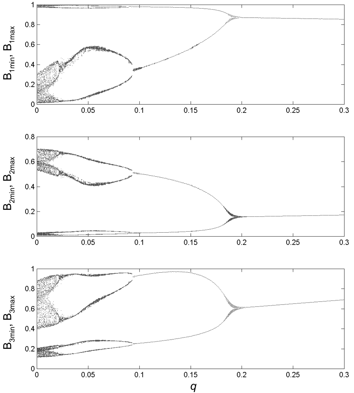
Figure 2. Local minima and maxima for each species in a three-species food chain for a range of values of q . Species 1 is the producer. The non-zero parameter values are x_1 = .4 , x_2 = .08 , y_{21} = 2.09 , y_{32} = 5 , a_{21} = 1 , a_{32} = 1 , e_{ij} = 1 , r_1 = 1 , K_1 = 1 , B_{012} = .16129 , B_{023} = .5 .
