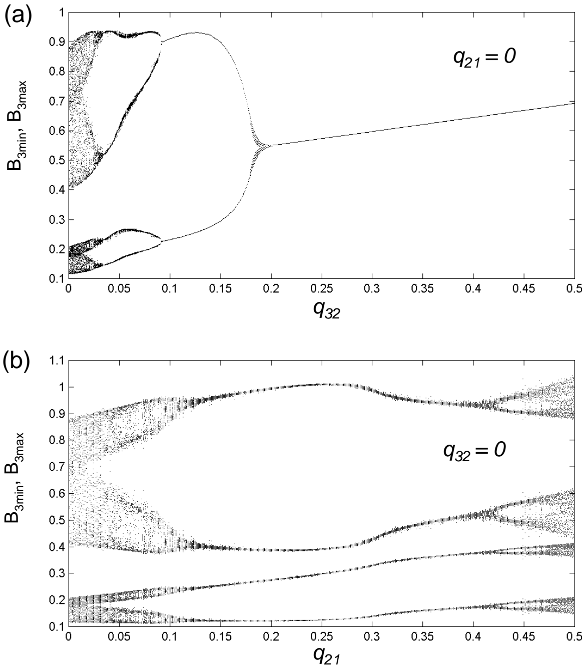
Figure 4. Local minima and maxima for the top species in a three-species food chain with one type II link and one type III link. The non-zero parameter values are as in figure 3: x_1 = .4 , x_2 = .08 , y_{21} = 2.09 , y_{32} = 5 , a_{21} = 1 , a_{32} = 1 , e_{ij} = 1 , r_1 = 1 , K_1 = 1 , B_{012} = .16129 , B_{023} = .5 . (a) The link between the top and intermediate species has type III functional response. (b) The link between the intermediate species and the producer species has type III functional response.
